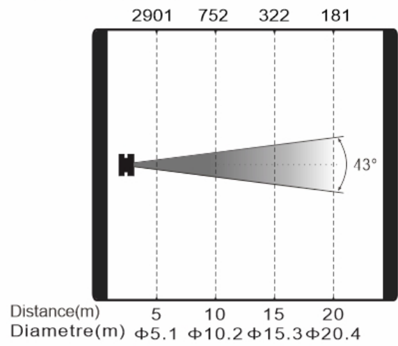
Max. Beam Mode Intensity LUX (43°)
